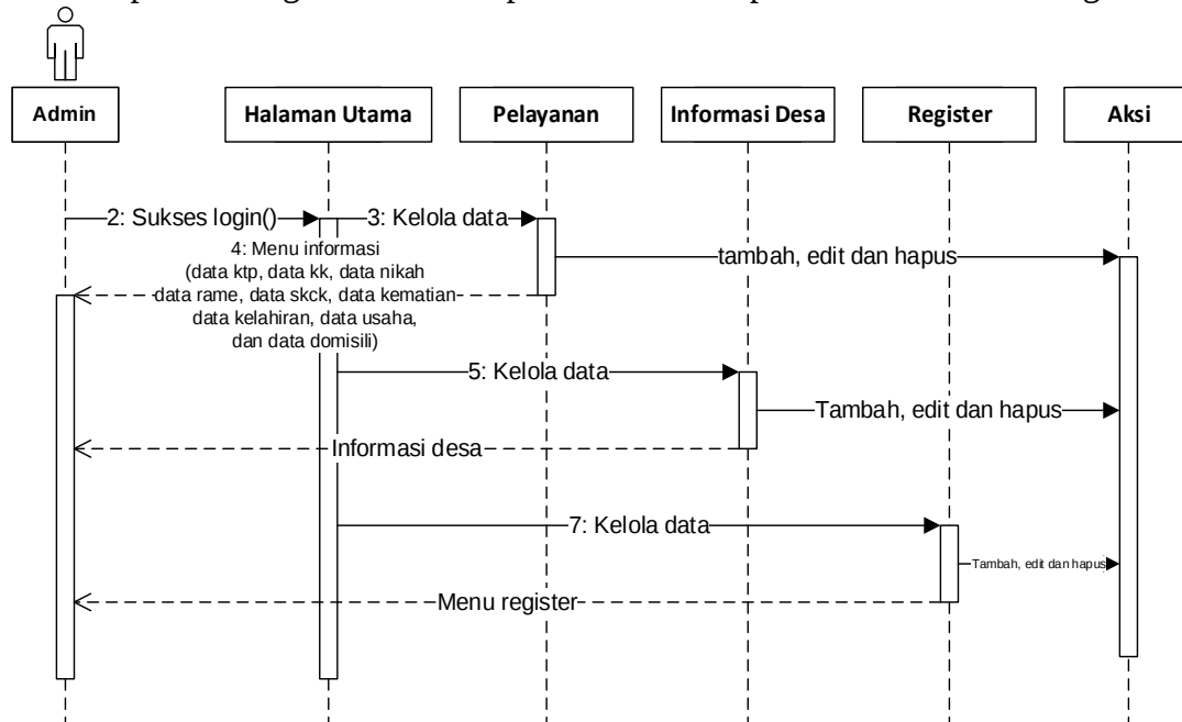
Gambar 2. Sequence Diagram Admin
