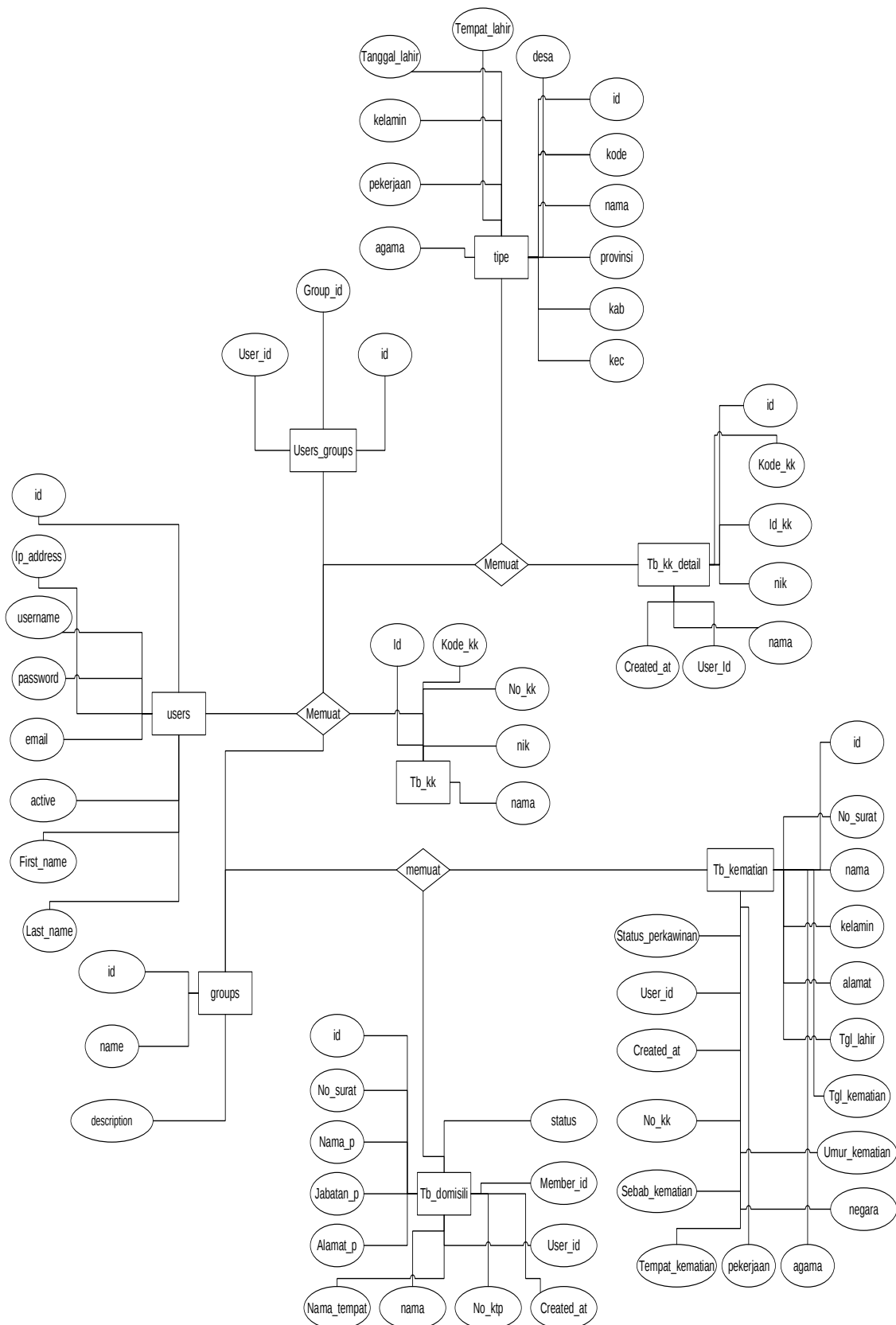
Gambar 4. Entity Relationship Diagram
