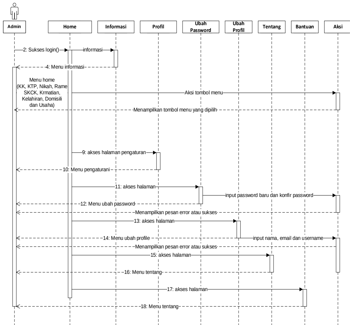
Gambar 3. Sequence Diagram User
